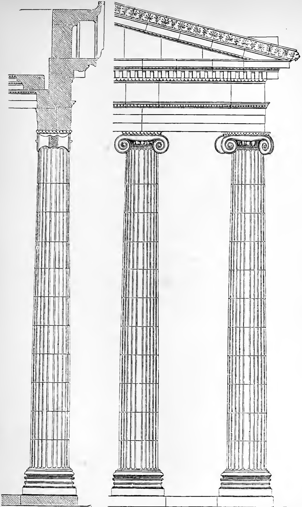
FIG. 70.—THE IONIC ORDER. FROM PRIENE, ASIA MINOR.
